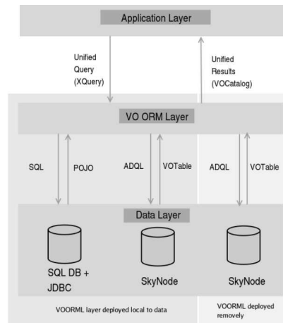
Figure 3. Detail of interaction between application, VOORML and data layers.
