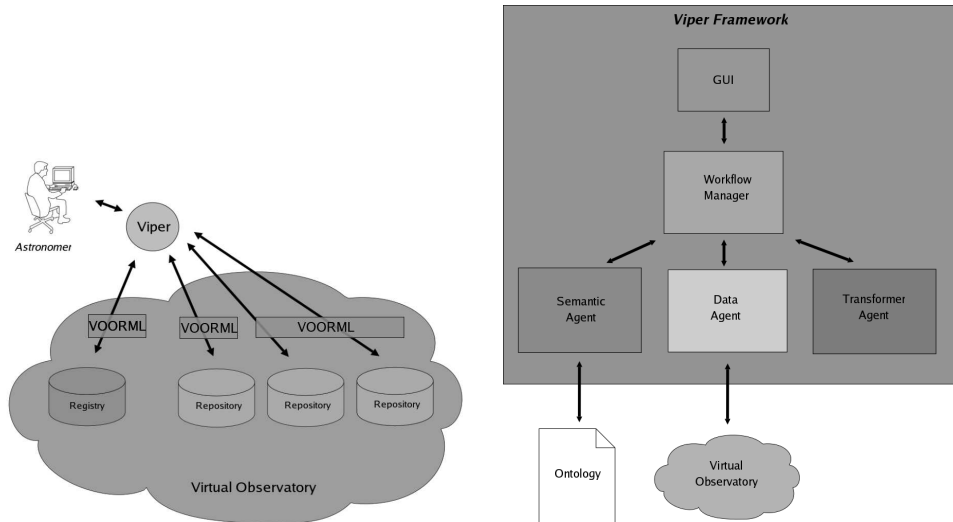
Figure 1. Summary of knowledge discovery framework. Left plot: The relationship between Human, VOORML, VO repositories and Viper. Right plot: major components of Viper tool.
