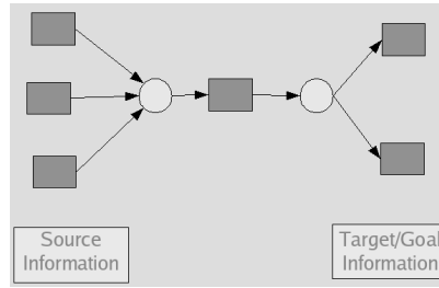
Figure 2. Viper workflow representation. Squares represent semantic objects and circles indicate relationships between them. The workflow allows the user to design information flows wherein “sources” at repositories are retrieved, and then transformed as desired into “goal” form.
